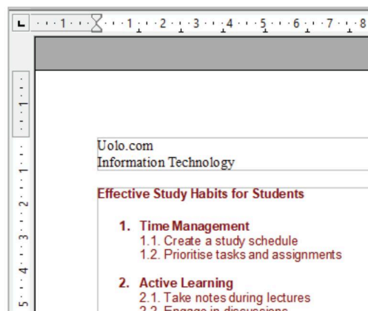
Fig. 6.32: Inserting Header
