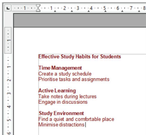
Fig. 6.21: Sample Text
