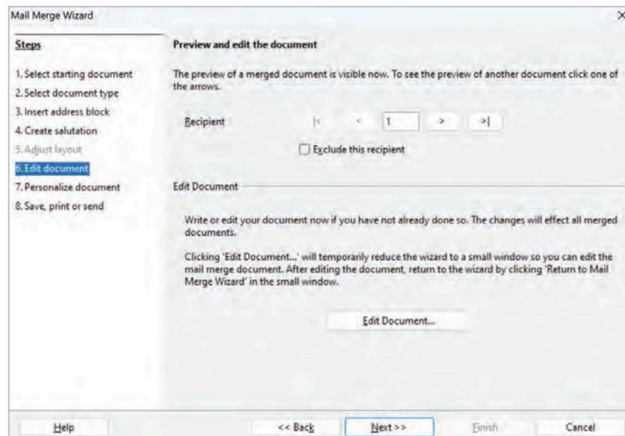
Fig. 9.16: Editing Document
