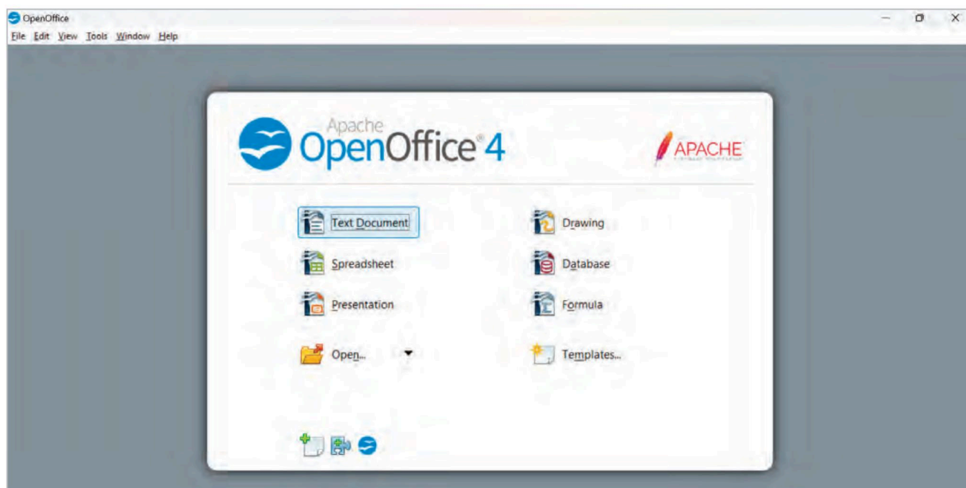
Fig. 4.1: OpenOffice Suite
