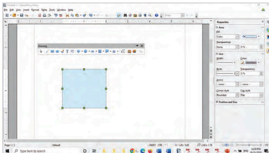
Fig. 6.38: Inserting Shape
