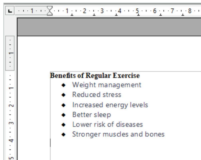
Fig. 6.20: Bulleted List
