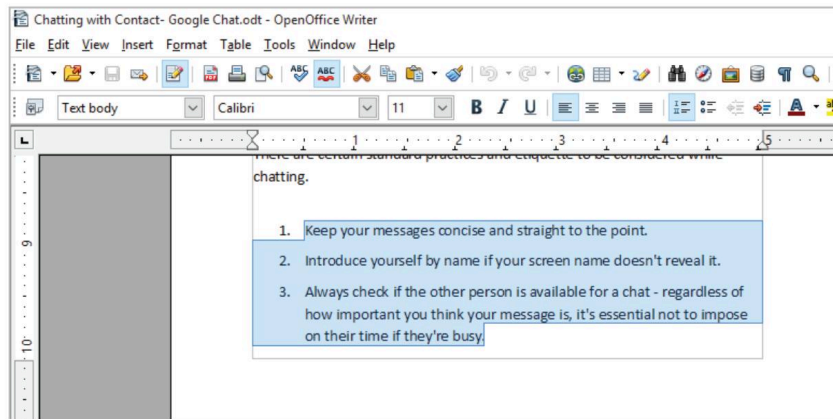
Fig. 6.5: Selecting Text
