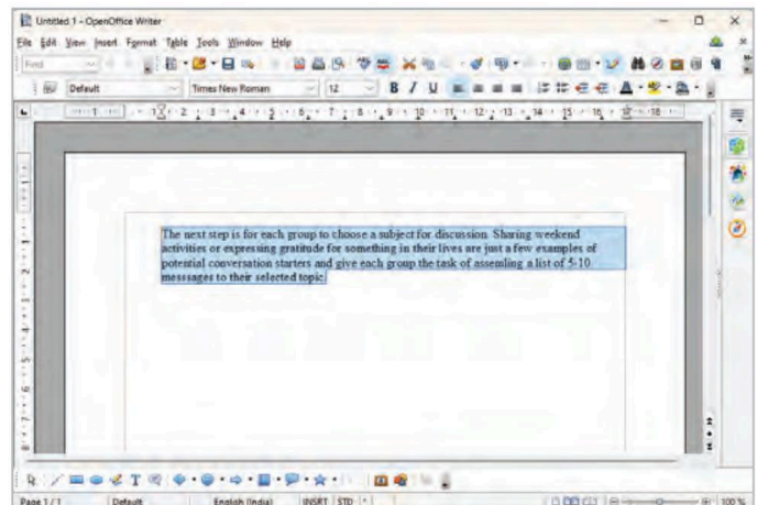
Fig. 6.11: Indented Paragraph
