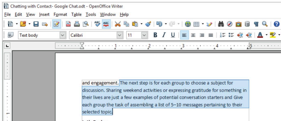
Fig. 6.24: Selecting Paragraph
