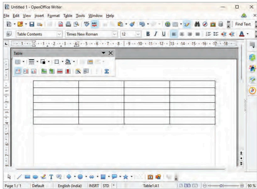
Fig. 7.5: Inserted Table
