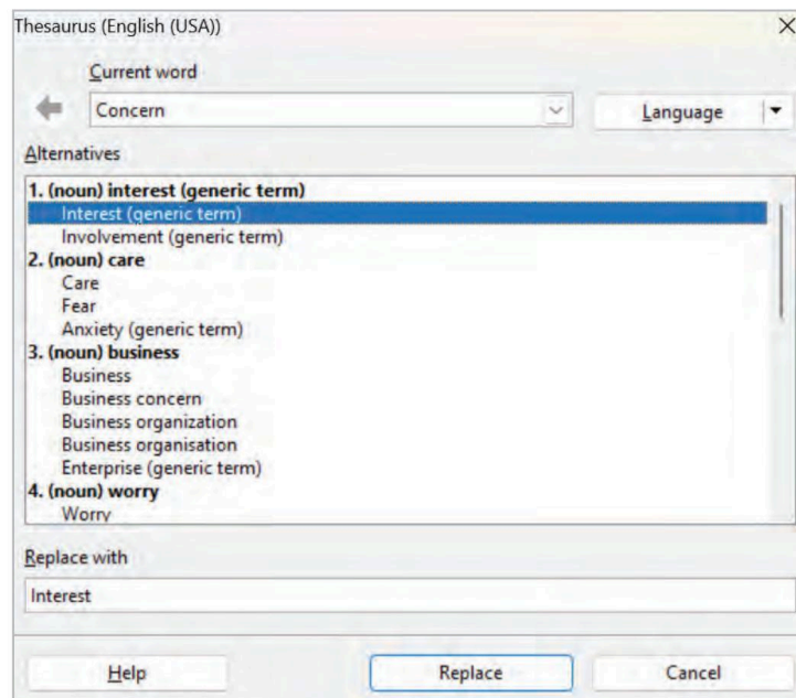
Fig. 5.14: Using Thesaurus
